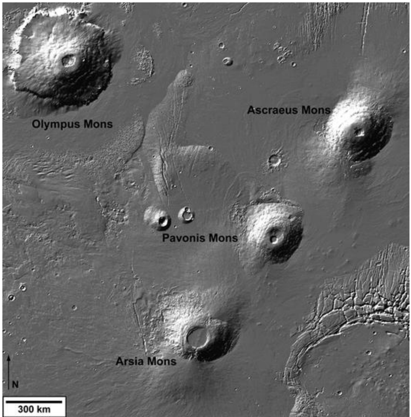
Shaded relief image of Tharsis Montes and Olympus Mons derived from Mars Orbiter Altimeter data which flew on board NASA's Mars Global Surveyor. The new data suggest that Tharsis Montes formed one by one, starting with Arsia Mons, possibly by the movement of a single mantle plume moving under the surface.
