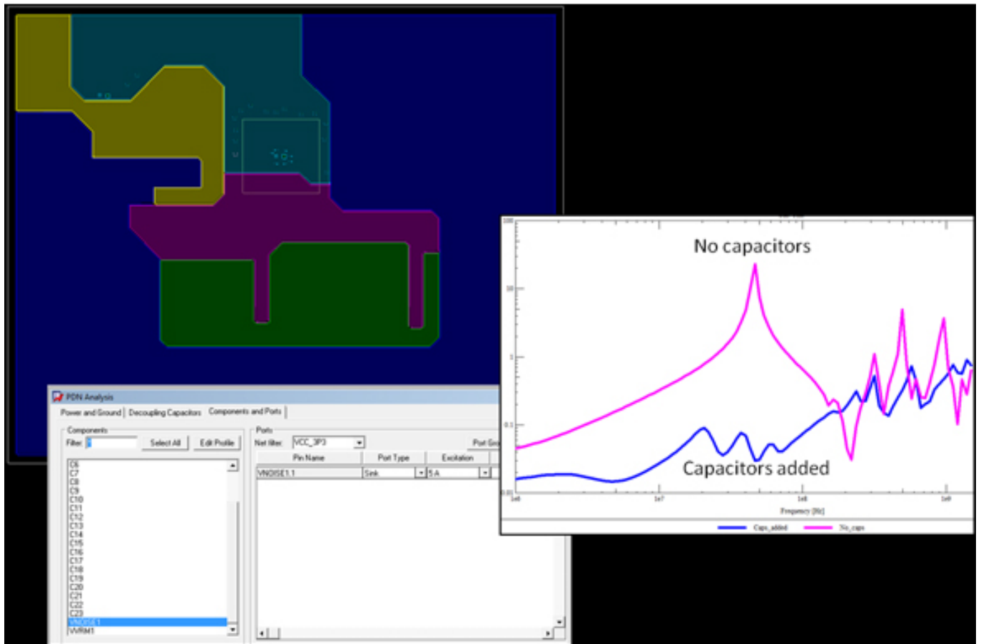
Figure 2: Early what-if analysis verifies capacitor selection, stackup, and plane splits. This can happen prior to a full netlist and should allow seamless transfer of design intent downstream.
