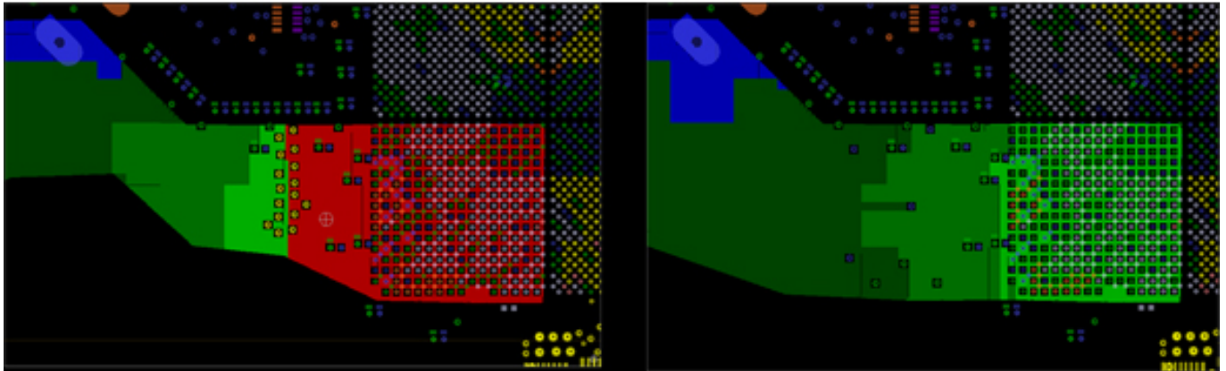
Figure 1: The picture on the left shows an area with an IR drop problem due to a via field and insufficient copper. The types of changes required are well suited to the PCB designer. If the reporting and editing are within the same canvas, the process of analyzing, editing, and re-analyzing can be very efficient.
