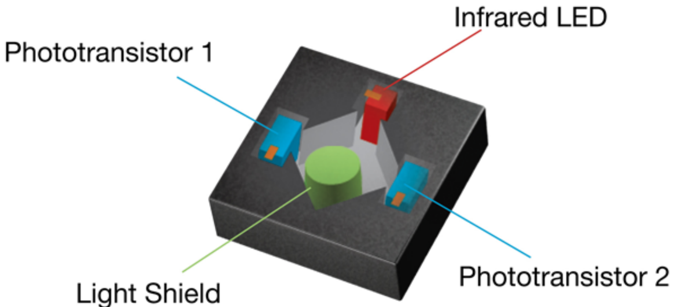
Figure 2. ROHM's RPI-1040 tilt sensor package includes a novel light shield that ensures silent operation, avoiding noise frequently exhibited by other designs during rotation.
