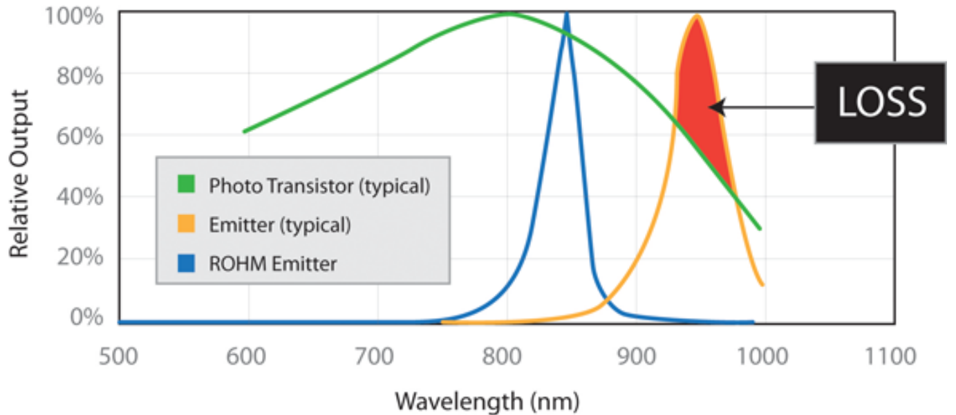
Figure 1. With peak output at 850 nm, high performance emitters such as ROHM Semiconductor’s SIM-041ST, operate much closer to the wavelength of phototransistors, resulting in reduced energy losses.
